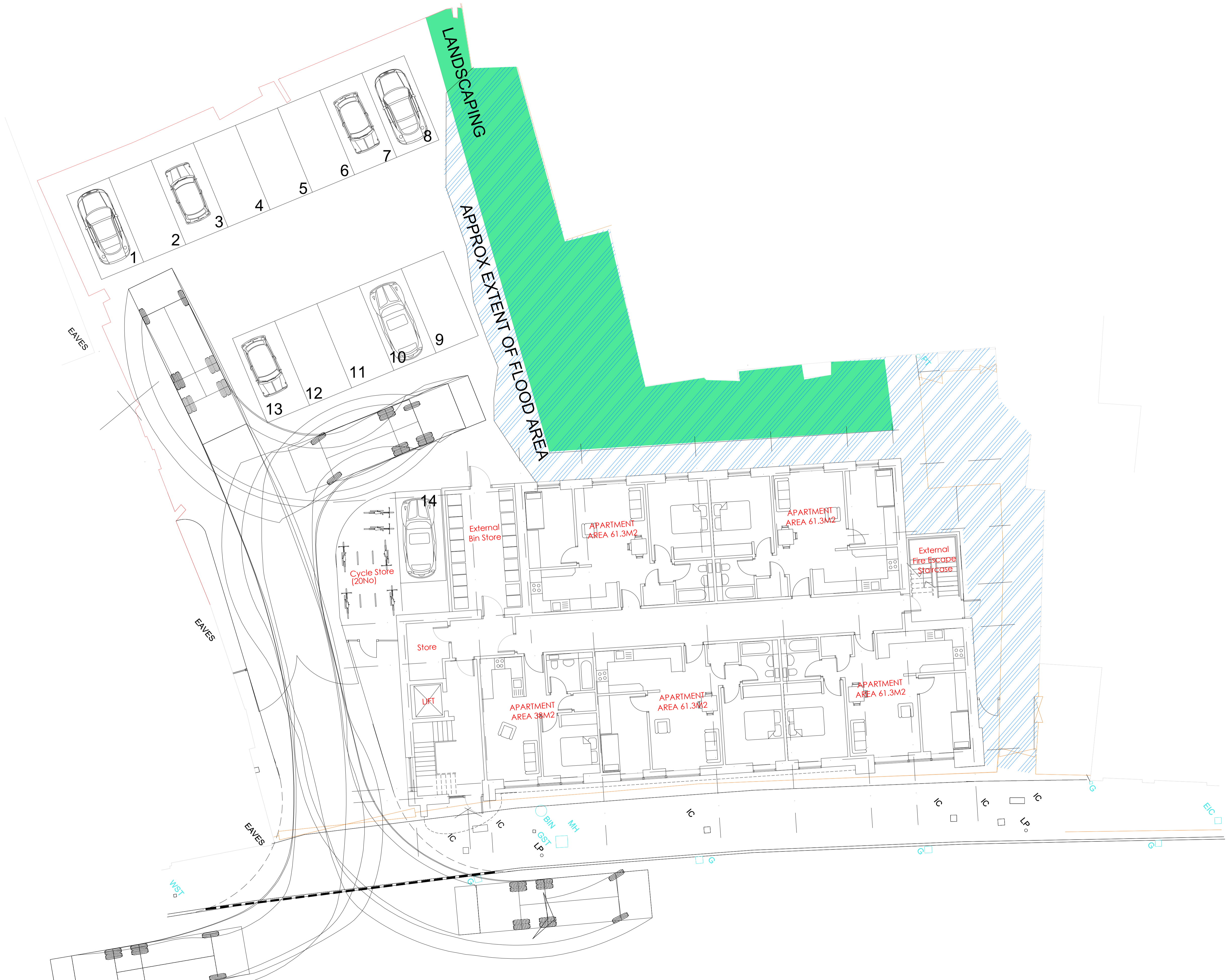
PROPOSED CAR PARK PLAN. 1:100
