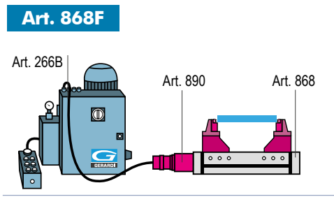
(Art. 868 + 890 + 266B) Morsa + motore idraulico + centralina / Vise + hydraulic motor + power unit
