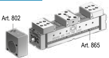
Double, single, self-centering FMS vise with quick change pull down jaws (comb system)
